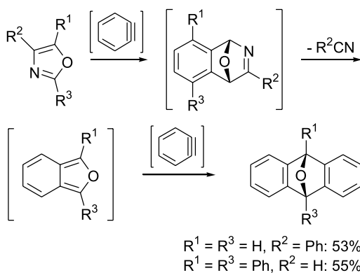
Scheme 22. Synthesis of bis(benzyne) adducts.
