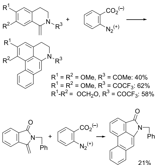
Scheme 32. Synthesis of dehydroporphines and aristolactams.
