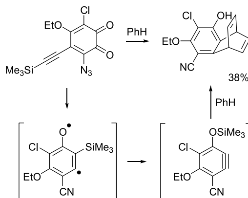
Scheme 9. Generation of arynes from azidoquinones.
