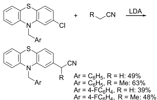
Scheme 89. Synthesis of 2-( \alpha -cyanoethyl)phenothiazines.
