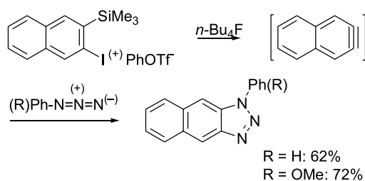
Scheme 63. Synthesis of 1-arylnaphtho[2,3- e ]triazoles.
