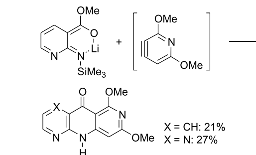
Scheme 68. Synthesis of azaacridones and diazaacridones.
