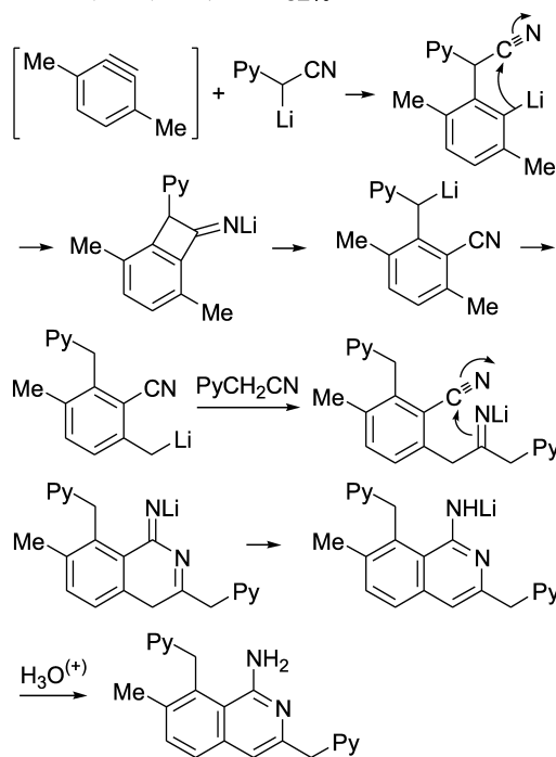
Scheme 88. Synthesis of aminoisoquinolines.
