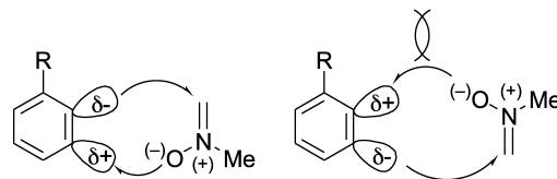
Scheme 61. Proposed explanation for the regioselectivity of the aryne–nitrene cycloaddition.
