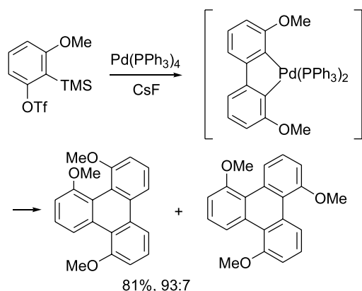
Scheme 105. High regioselectivity explained by a metallacyclic intermediate.
