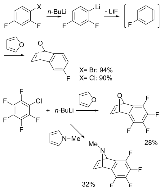
Scheme 17. Synthesis of fluorinated benzonorbornadienes.
