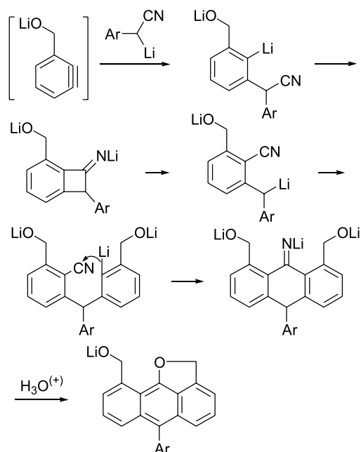
Scheme 87. Synthesis of 1-hydroxymethyl-6-aryl-2H-anthra[9,1-bc]furans and the proposed mechanism.
