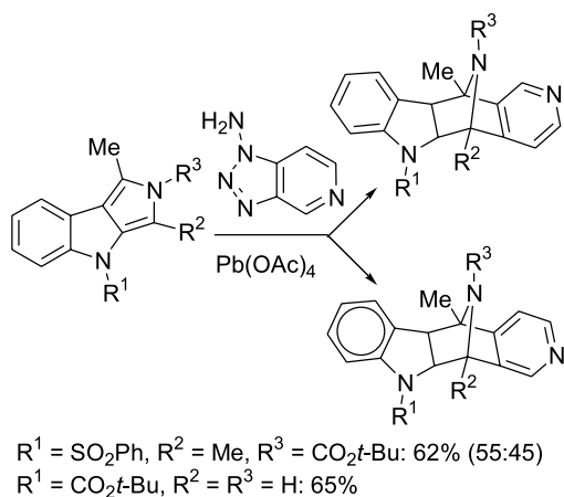
Scheme 29. Synthesis of indoles.
